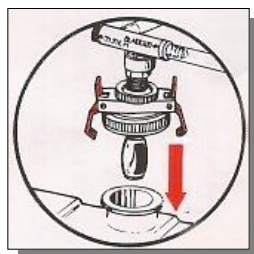
Mounting the Universal Adaptor to Radiator Neck
